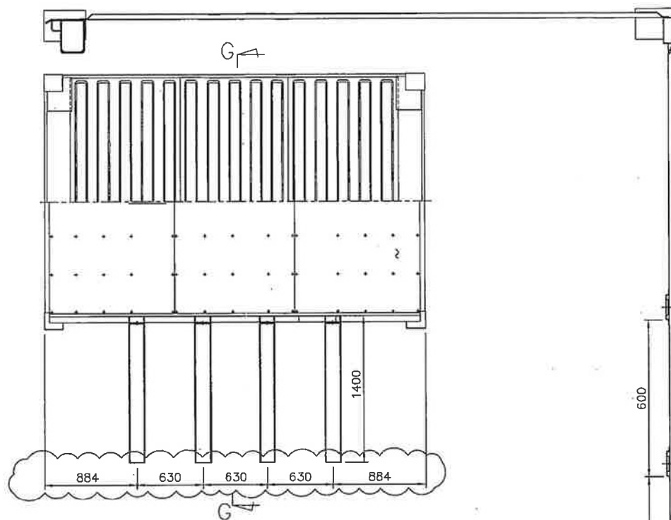
ROLL RAIL TOP VIEW
