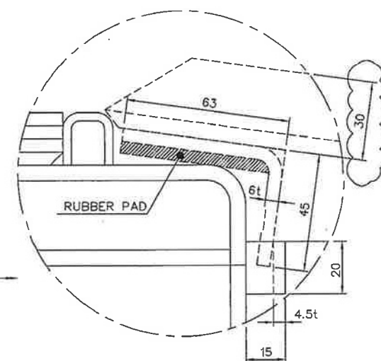
DETAIL E-E
